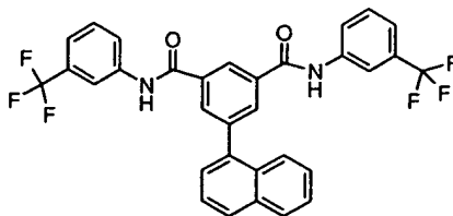
Compound # 3
